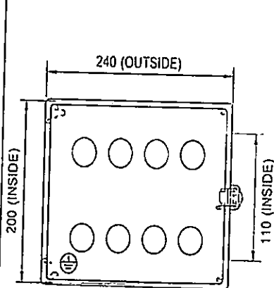
PLAN VIEW (WITHOUT CLAMP)
