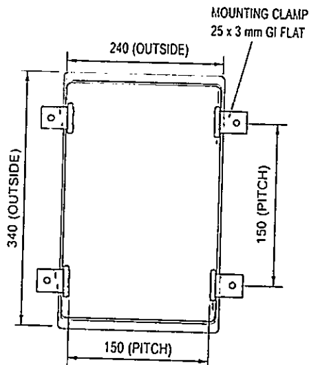
PLAN VIEW (WITH MOUNTING CLAMP)
